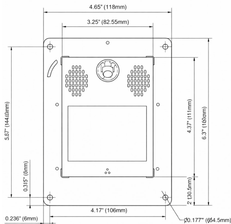
7200 Elevator Unit
