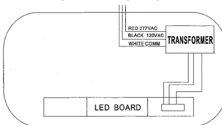
AC ONLY WIRING DIAGRAM
