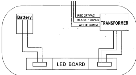
BATTERY BACKUP WIRING DIAGRAM
