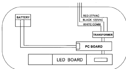
SELF DIAGNOSTIC WIRING DIAGRAM
