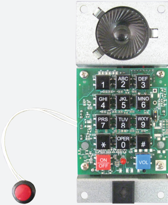
Part #: 2400-875HE Dimensions: 6-1/2" H x 3" W x 3/4" D Style: Interior Speaker Phone, Behind the Panel Mount
