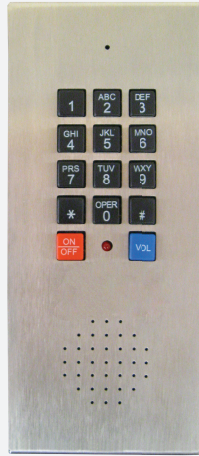
Part #: 2400-876HE Dimensions: 8-3/8" H x 3-5/8" W x 1-1/8" D Style: Interior Speaker Phone, Box Style/Surface Mount
