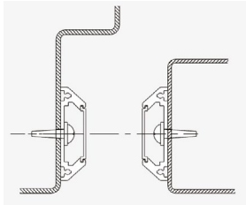
744 XXX (2m / 2.1m) Self-Tapping Screw
