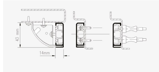
744 040 Self-Tapping Screw or Wing nut fixing for Slampost
